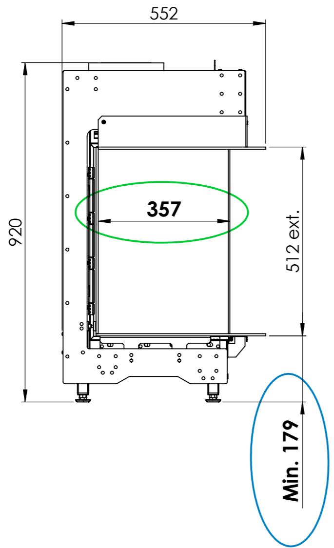
MatriX 1050x500 I, II, III (Logburner 2.0)
